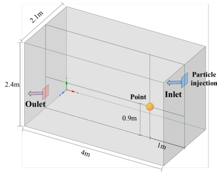
Fig. 2 Configuration of the chamber and measuring point location.
